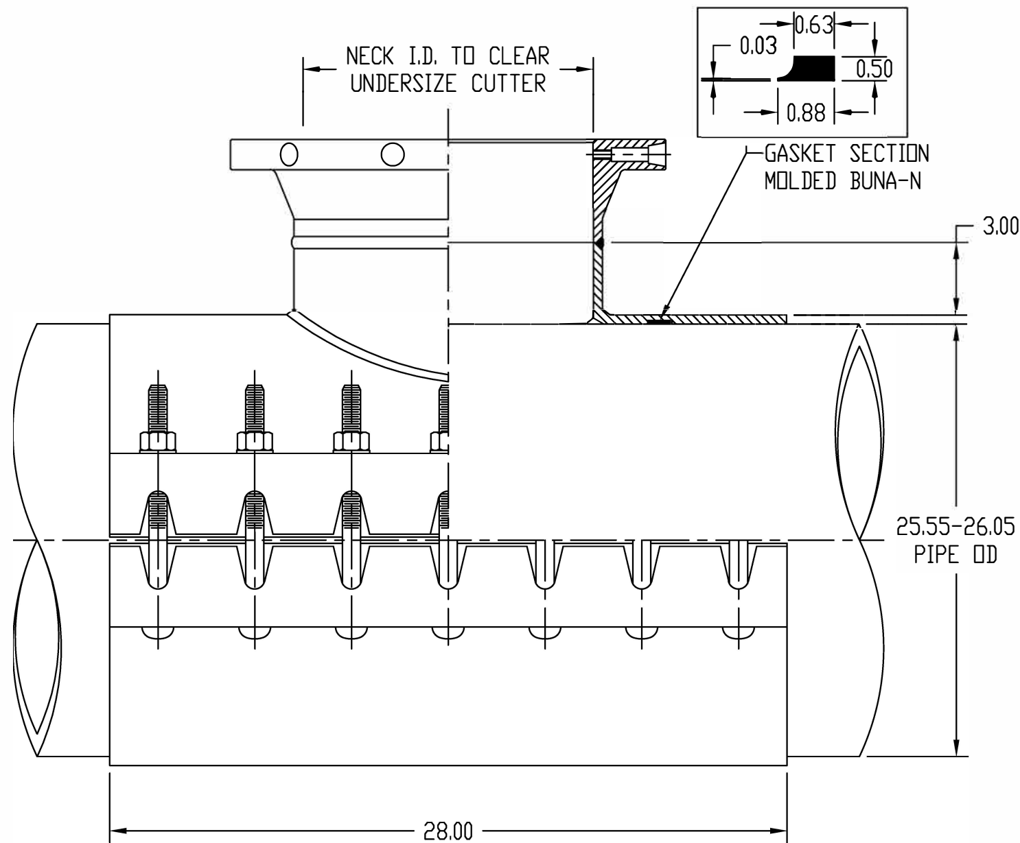
SECTION
