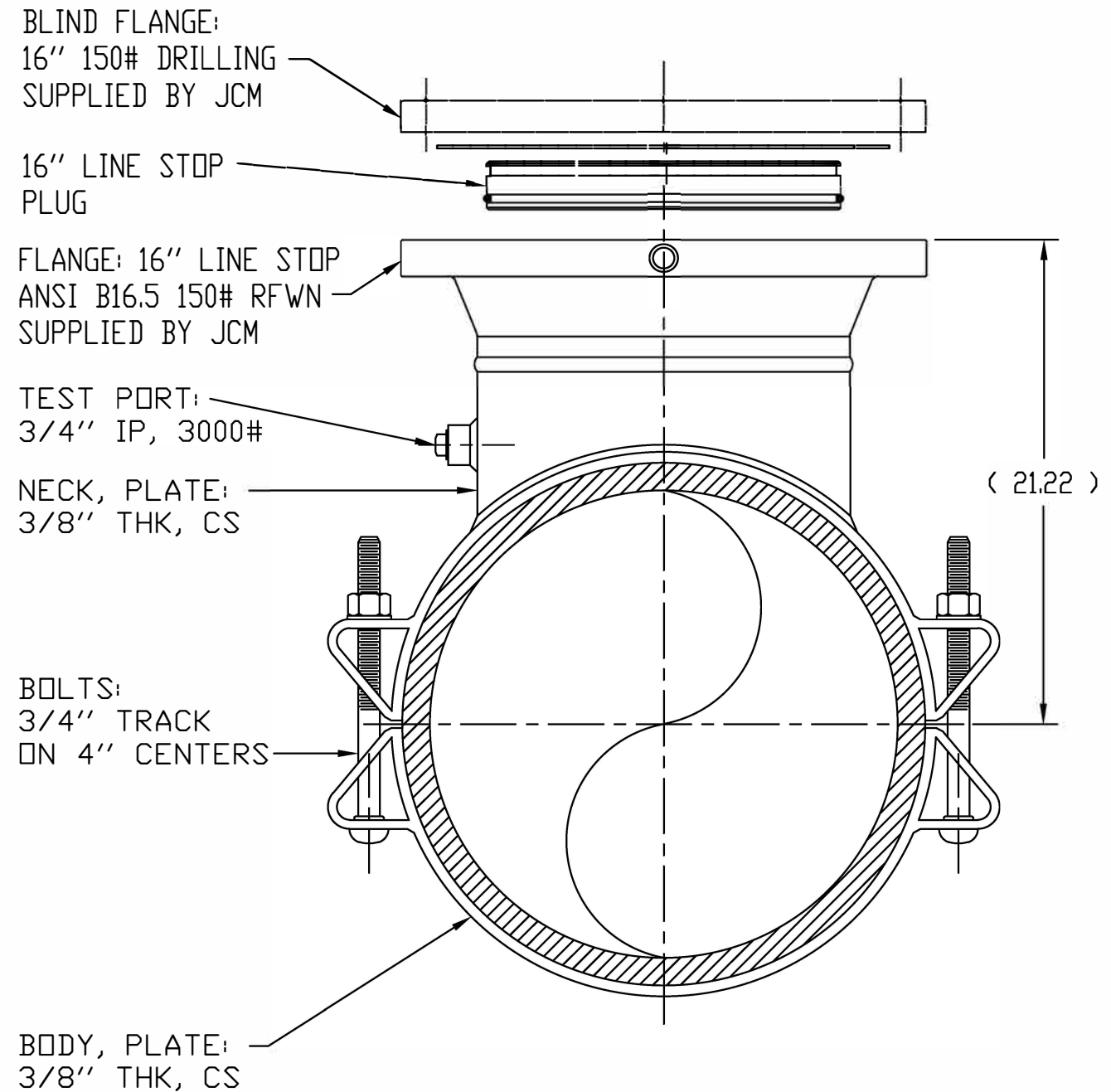
END VIEW
